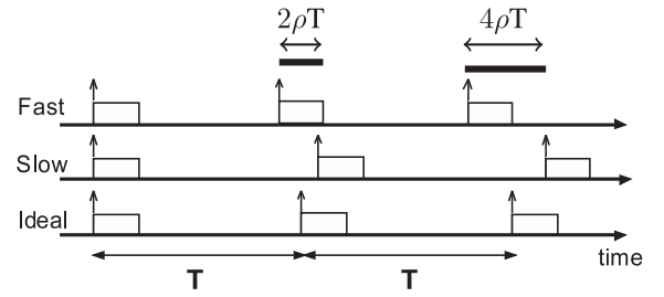
Fig. 7. Possible behavior of three nodes executing Task1 (drifting computer clocks).
