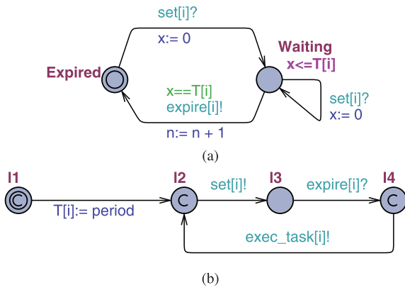
Fig. 14. The two UPPAAL templates used for specifying the system: (a) corresponds to an ideal timer of period T , whereas (b) corresponds to the application.
