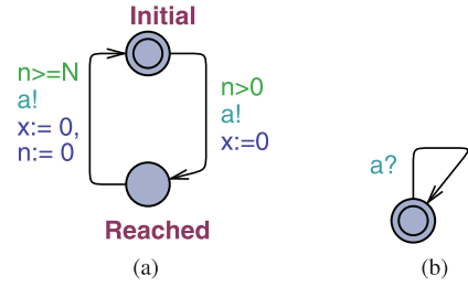
Fig. 18. The two timed automata used for verifying the precision: (a) the observer, (b) a dummy automaton required for the evolution of the observer.
