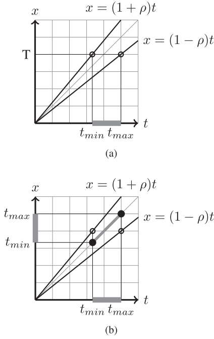
Fig. 11. A timer that measures T t.u., with drift \rho : (a) the location of the expiration interval, (b) the mapping to an ideal clock.
