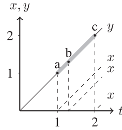
Fig. 2. Possible behavior of TA A_1 , with three potential traces.
