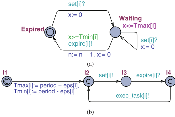
Fig. 15. The two UPPAAL templates used for specifying the system with drifting clocks: (a) the timer, which corresponds to a perturbed timed automata, whereas (b) models the application (Task1).
