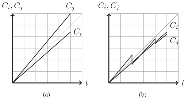
Fig. 4. Evolution of two computer clocks: (a) drifting clocks; (b) with clock synchronization.
