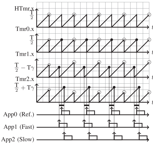
Fig. 21. Possible behavior of a system with synchronized clocks.
