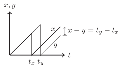
Fig. 3. Representation of the temporal evolution of two TA clocks.
