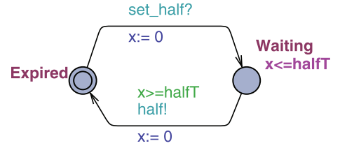
Fig. 16. Template of the clock pointer. It is named Half_Tmr because it measures half of the round duration.
