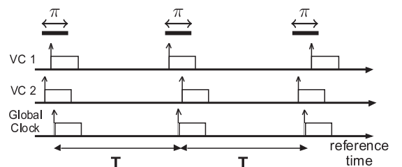
Fig. 8. Possible behavior of three nodes executing Task1 (synchronized computer clocks).
