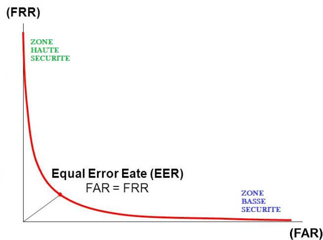
Fig 1.6 – Courbe ROC [Ijiri et al., 2012]
