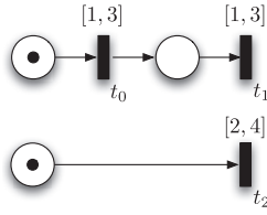
Fig. 2. The pSTPN model of two concurrent activities.
