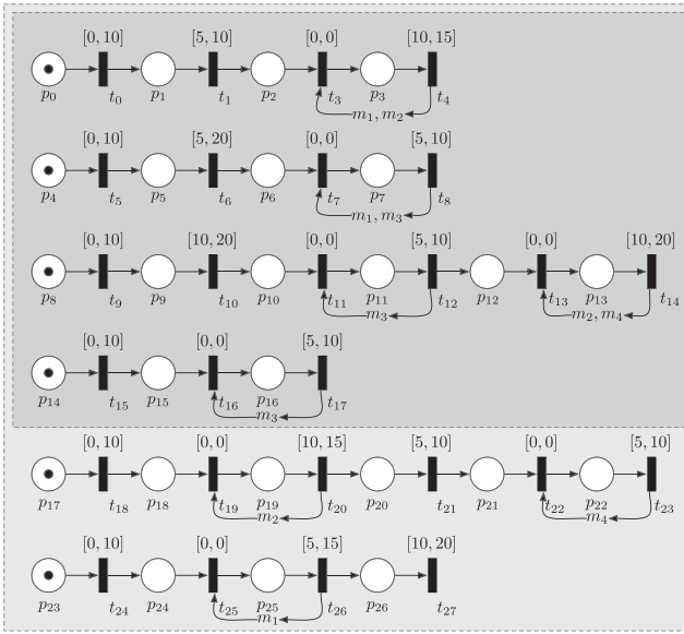
Fig. 8. pSTPN models of a task set made of four tasks (inner box) and six tasks (outer box), synchronized on four mutually exclusive resources. Places accounting for mutual exclusion among chunks are omitted for readability and substituted by their names m_1, \dots, m_4 .
