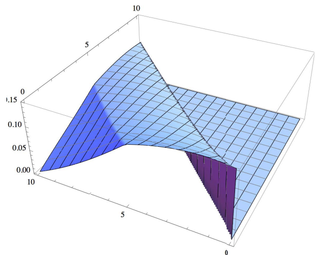
Fig. 6. (a) The DBM zones that constitute the partitioned domain of function P_{OK}(x_0^0, x_1^0) , representing the probability of execution of the run \rho_2 = t_0 \rightarrow t_5 \rightarrow t_1 \rightarrow t_3 \rightarrow t_6 \rightarrow t_4 \rightarrow t_7 \rightarrow t_8 as a function of controllable transitions t_0 and t_5 , in the example of Fig. 5. (b) Plot of function P_{OK}(x_0^0, x_1^0) .
