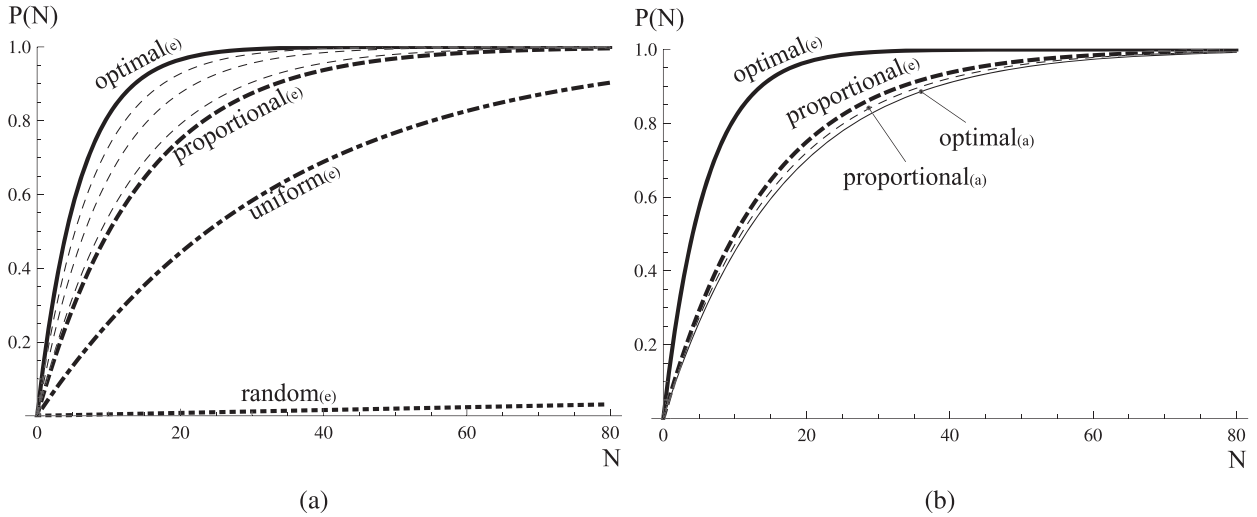
Fig. 7. (a) Probability of conclusive test execution as a function of the number of test repetitions, with optimal sampling (continuous thick line), proportional sampling with order k = 1, 2, 5, 10 (dashed lines, bottom-up for increasing values of k ), uniform sampling (dot-dashed thick line), random testing (dotted thick line). (b) Comparison of optimal sampling (continuous thick line) and proportional sampling (dashed thick line) based on exact estimates of function P_{OK}() (marked by subscript “(e)”) with respect to the approach of [43] (continuous thin line) and its combination with proportional sampling (dashed thin line), which are based on approximate estimates of P_{OK}() (marked by subscript “(a)”).
