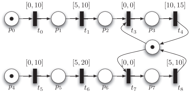
Fig. 5. psTPN model of the task set made of two tasks specified in Table 1.
