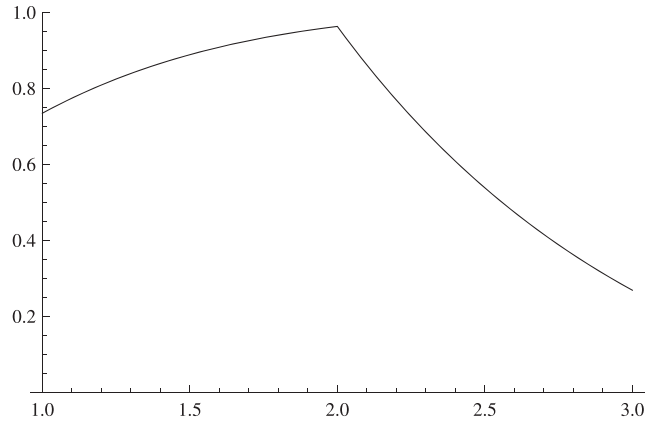
Fig. 3. The plot of function P_{OK}(r_{l(0,0)}) representing the probability of execution of the sequence \rho = t_0 \rightarrow t_2 \rightarrow t_1 in the example of Fig. 2 as a function of the firing-time r_{l(0,0)} of controllable transition t_0 .
