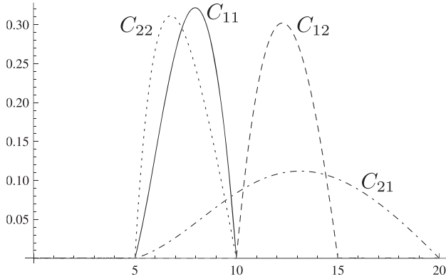
Fig. 4. Plot of the execution time distributions for the four chunks in Table 1.
