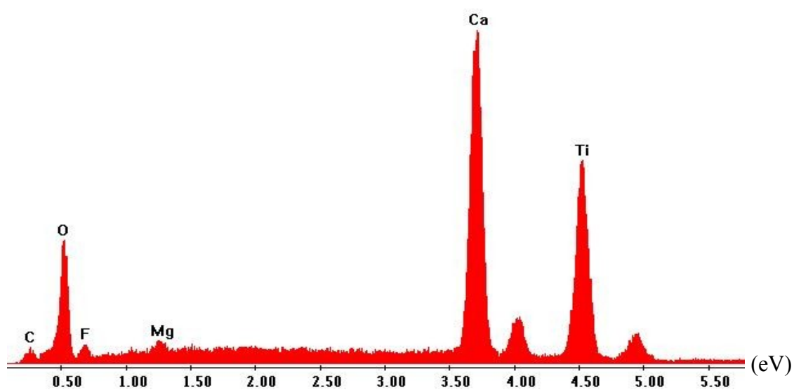
Figure 23: Spectre de microanalyse de la phase Ca_{0,90}Mg_{0,10}(Ti_{0,90}Li_{0,10})O_{2,70}F_{0,30}
