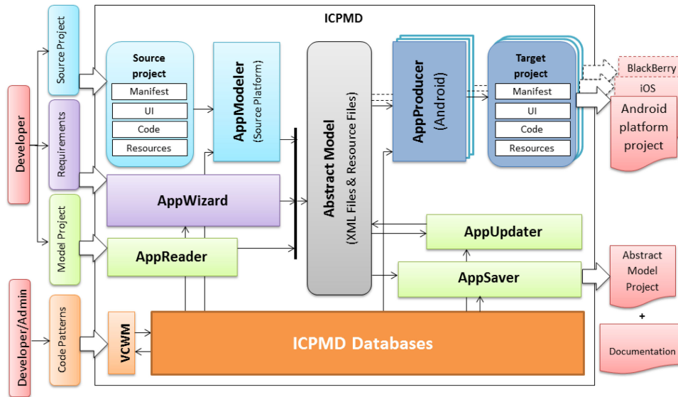
Fig. 1. The architecture of the ICPMD solution [24].
