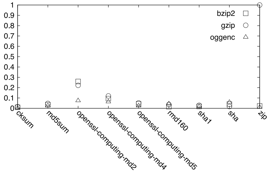
Fig. 6. Similarity scores (y-axis) between different programs (x-axis).
