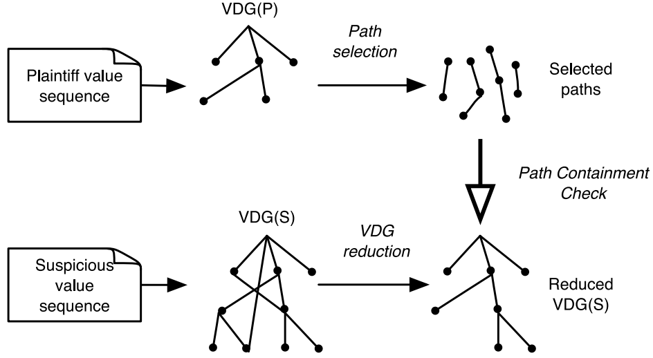
Fig. 7. VDG based detection overview.
