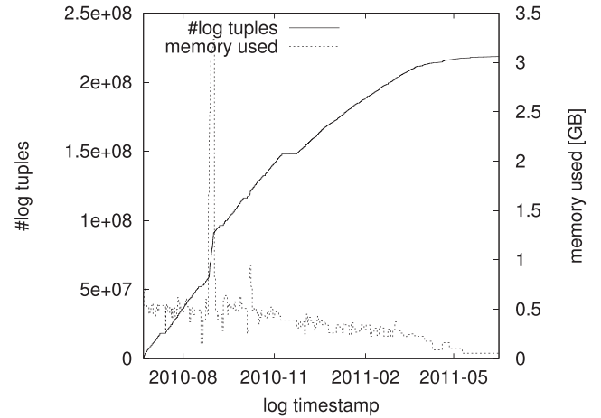
Fig. 9. Monitor memory usage on policy del-1-2 .
