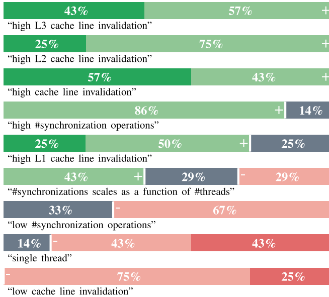
Fig. 8. Levels of experts' agreement on observations related to the "True sharing of updated data" problem.
