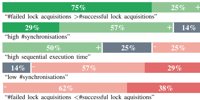
Fig. 3. Levels of experts' agreement on observations related to the “Lock contention” problem.
