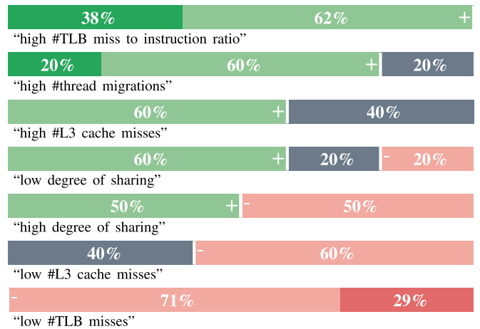
Fig. 13. Levels of agreement on observations related to the "TLB Locality" problem.
