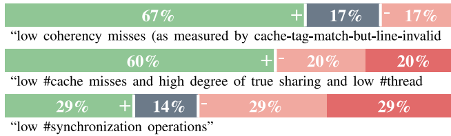
Fig. 7. Levels of agreement on observations related to the "Chains of data dependencies, too little parallelism" problem.
