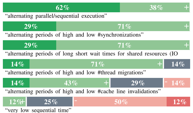
Fig. 6. Levels of experts’ agreement on observations related to the “Alternating sequential/parallel execution” problem.
