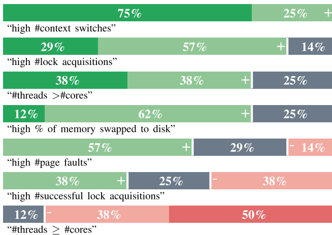
Fig. 10. Levels of agreement on observations related to the "Oversubscription" problem.
