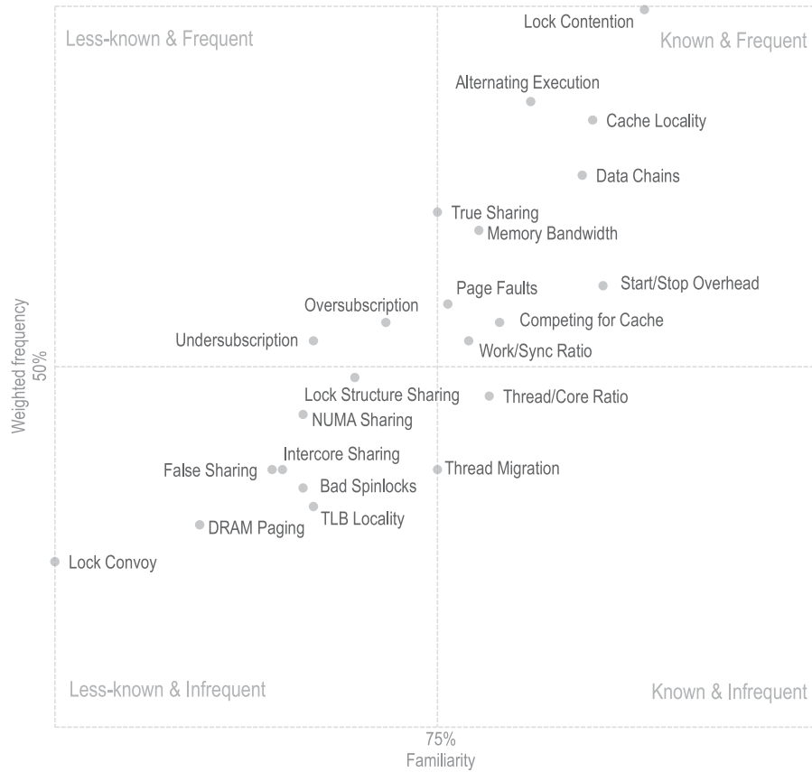
Fig. 4. Quadrant plot of parallel performance problems mapped against familiarity and frequency.
