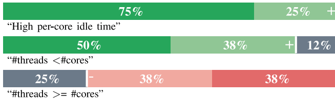
Fig. 9. Levels of agreement on observations related to the "Undersubscription" problem.
