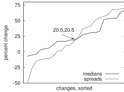
Fig. 11. Range of changes in median and spread generated by applying the recommendations of W2. The median observed changes were 20.5 and 20.5 percent for medians and spreads, respectively.
