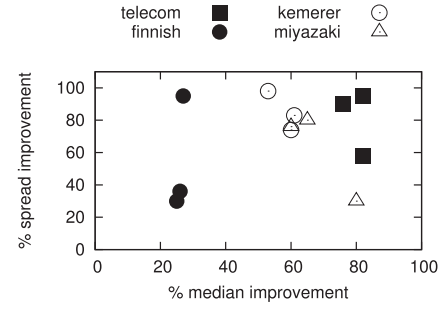
Fig. 8. Effort improvements for four data sets.
