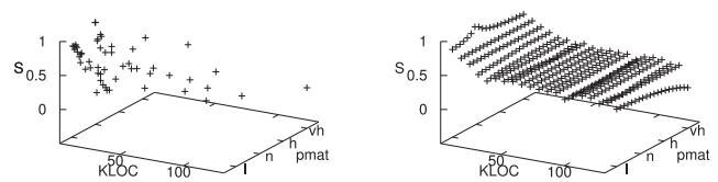
Fig. 1. In data farming, past project data (shown on left) is used to develop a software process model. This model is then executed to generate a landscape of possibilities (on right). In this figure, pmat is process maturity, KLOC is lines of code, and “ S ” is a score function that rewards projects with low defects and fast development times (so larger “ S ” scores are better ). For an example of this function, see (1), shown later in this paper.
