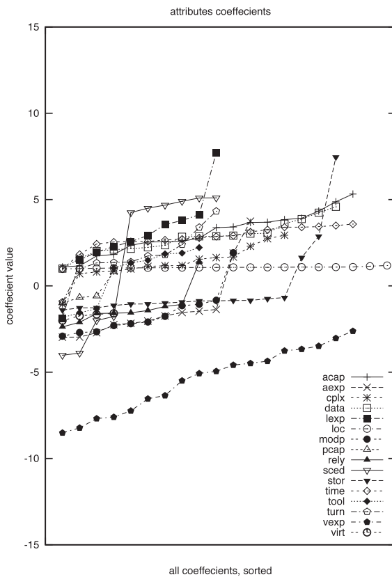
Fig. 12. COCOMO 1 effort multipliers and the sorted coefficients found by linear regression from twenty 66 percent subsamples (selected at random) from the NASA93 PROMISE data set [79]. Prior to learning, training data were linearized in the manner recommended by Boehm ( x was changed to \log(x) ); for details, see [79]). During learning, a greedy back-select removed attributes with no impact on the estimates: Hence, some of the attributes have less than 20 results. After learning, the coefficients were unlinearized.
