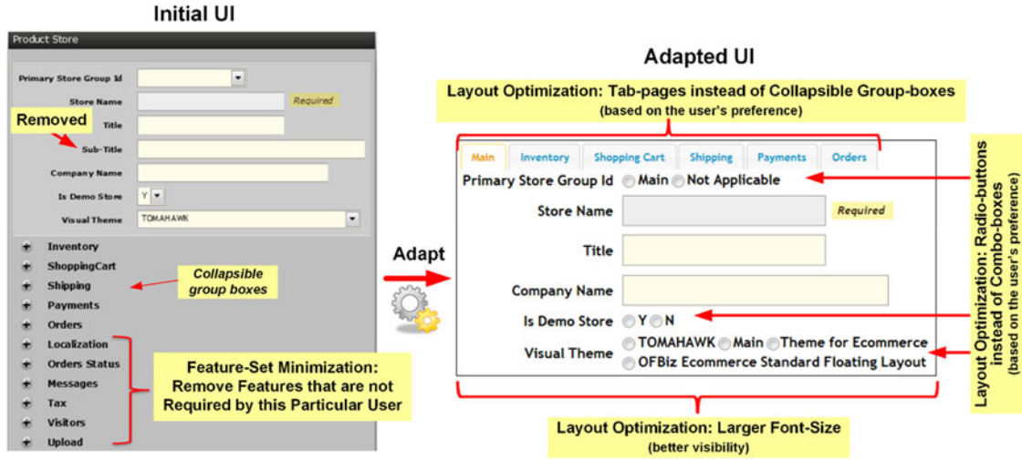
Fig. 1. An example on adapting a user interface with RBUI by minimizing its feature-set and optimizing its layout.
